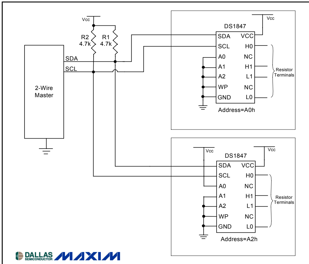
Figure 2. 2-Wire Interface
