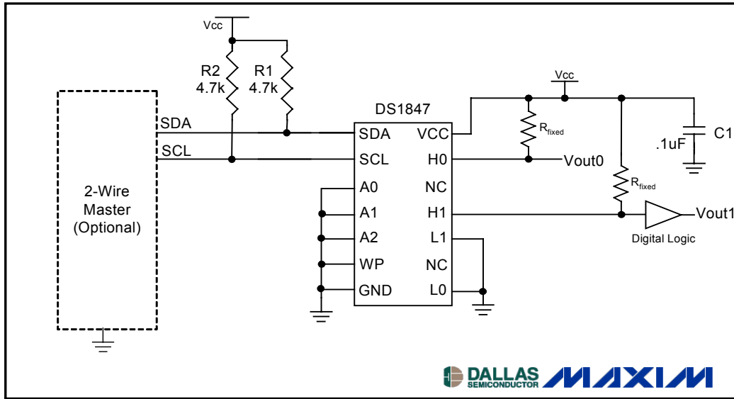
Figure 4. Voltage and Digital Outputs
